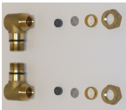
BO91242 - Concealed Elbow (Pair)
