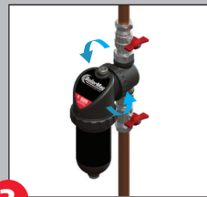
3 Fit BoilerMag
